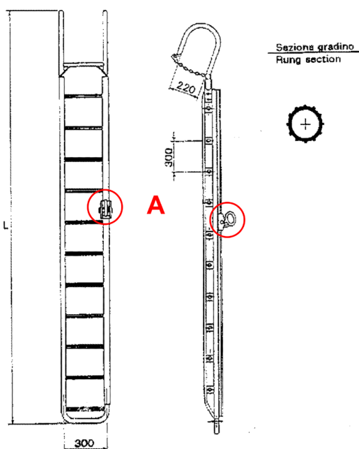
version AS with single antifall device
